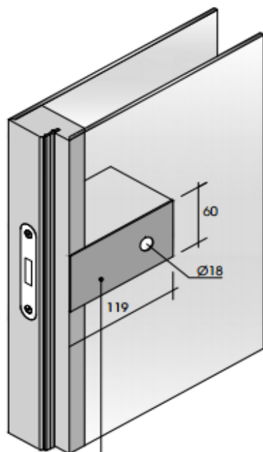
Particolare supporto serratura per Porta Pannellata Detail for handle support for paneled door
