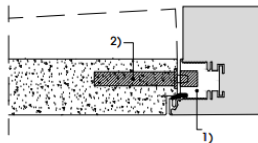
ELECTRICAL OPENING for Push and Pull doors - replacing to electromagnetic-lock
